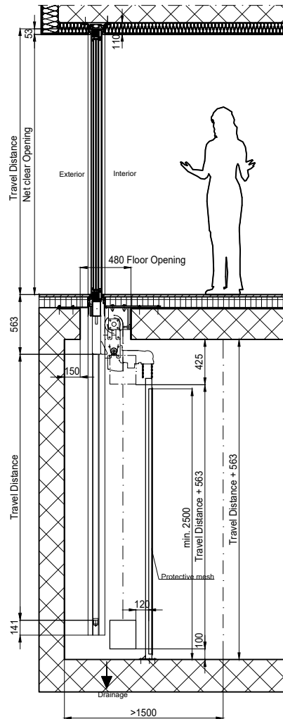
V-V Vertical Section, Mechanical Room
